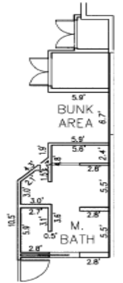
Unit Plan
